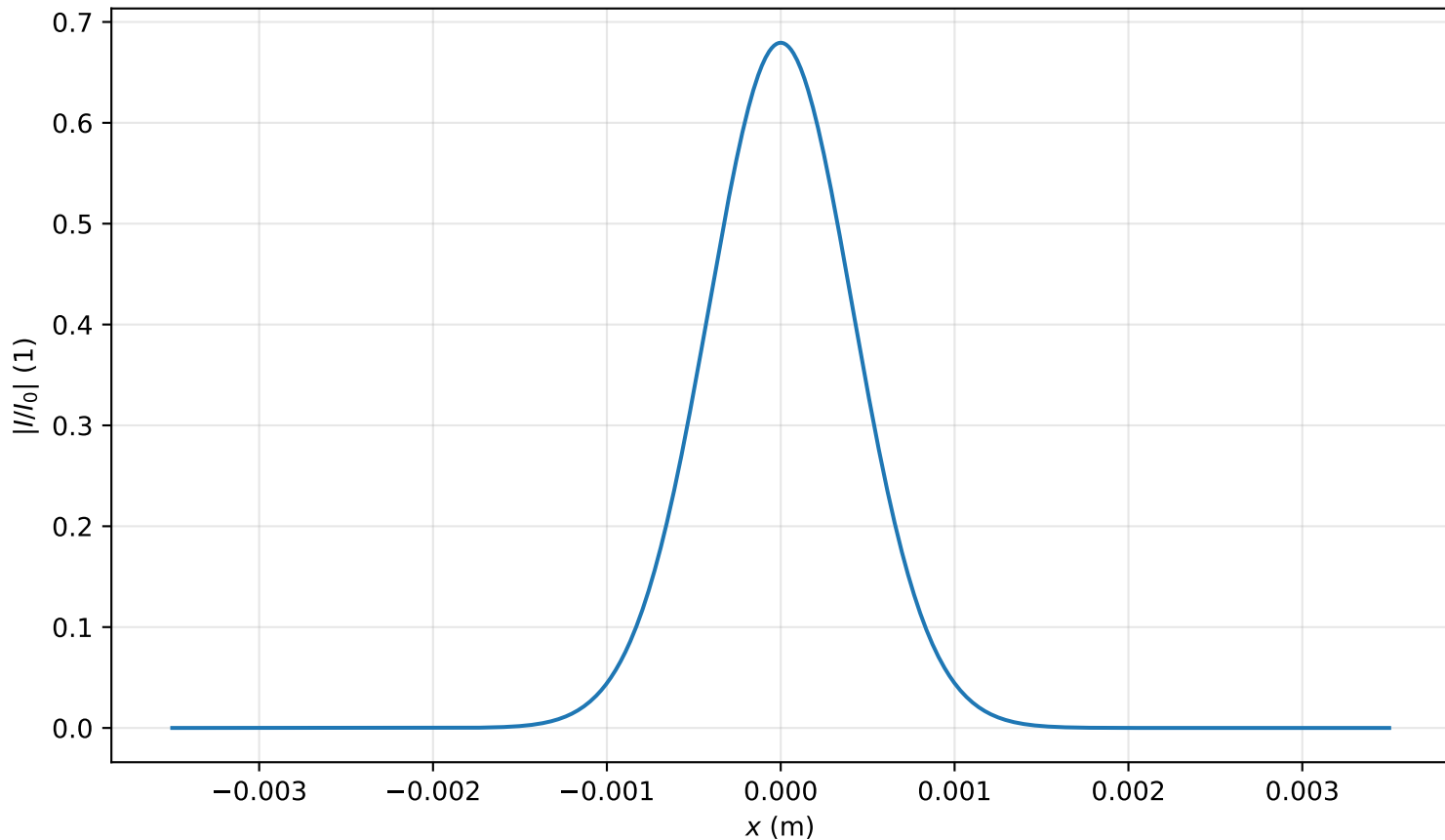
Intensity profile I(x, y = 0, z = 1.513m)/I_0 , P_{in}=0.1P_{cr} , artificial time
